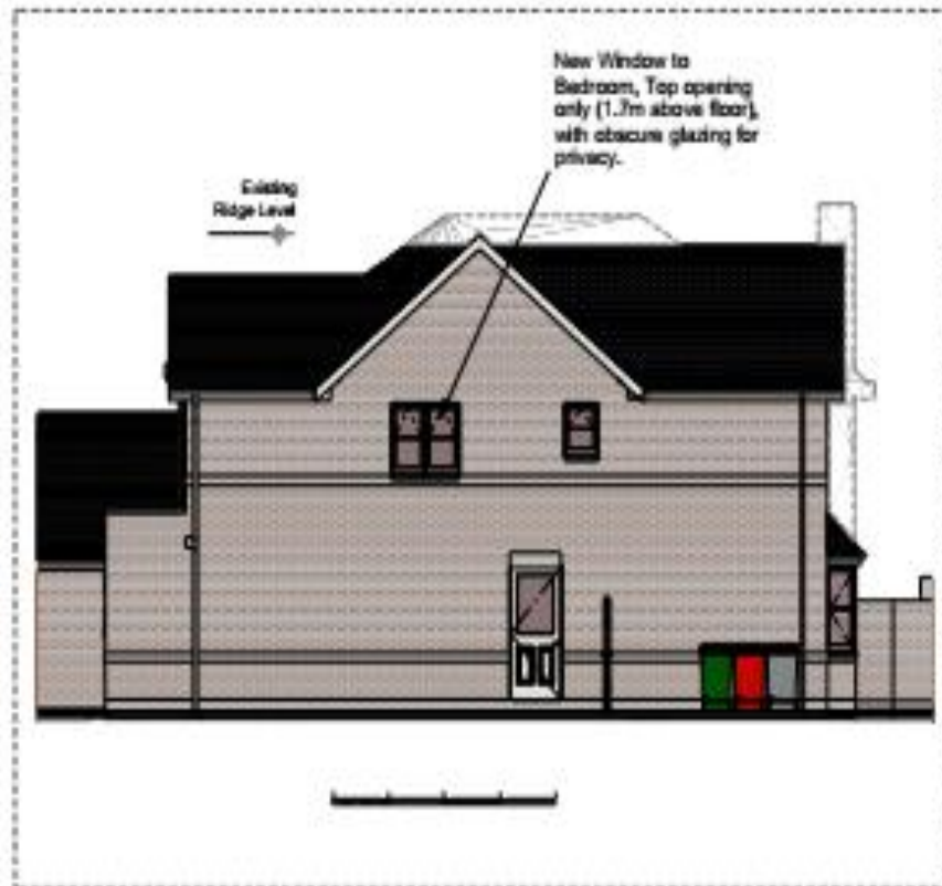
PROPOSED SIDE ELEVATION (LOOKING EAST)
